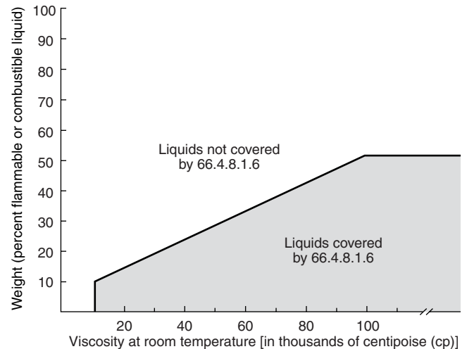
FIGURE 66.16.2.5 Viscous Liquid: Viscosity Versus Weight Percent Flammable or Combustible Component. [30: Figure 16.2.6]
