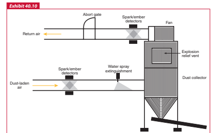
Basic spark detection and extinguishment system for a single air-material separator.
