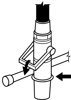
FIGURE A.13.6.4.7.2(e) Nozzle in Holder. [10:Figure A.7.7.1.1(e)]
