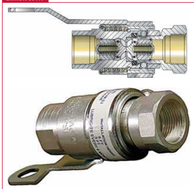
Pull-away valve. (Courtesy of RegO® Products)
