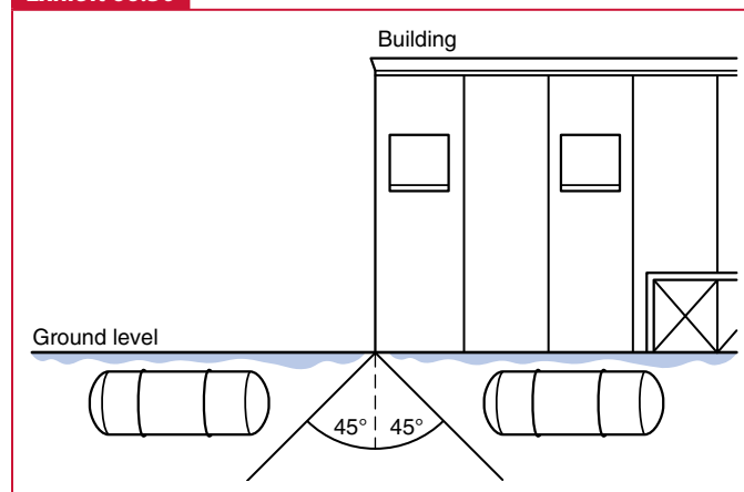
Siting of underground tanks with respect to building footings and foundations.
