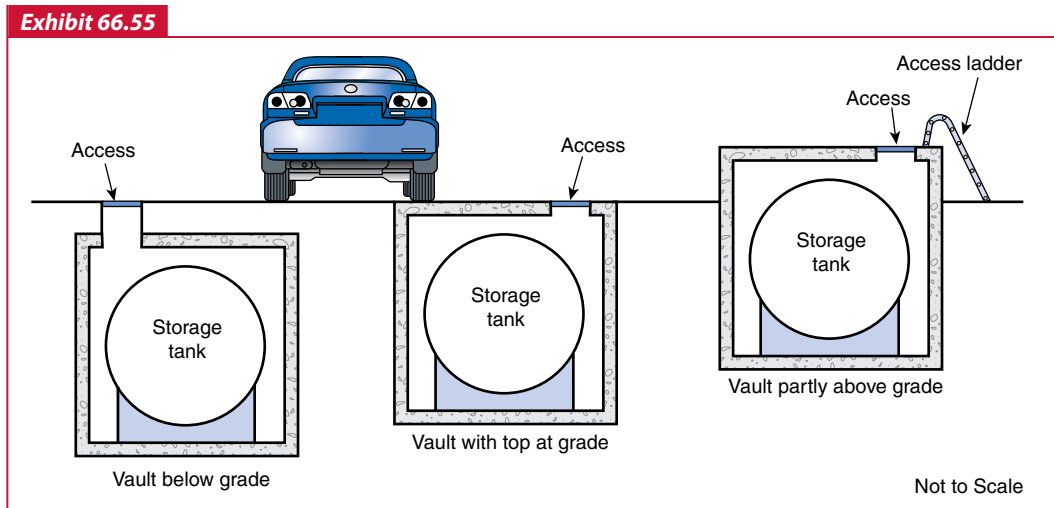
Diagram showing vault installations with respect to grade.
