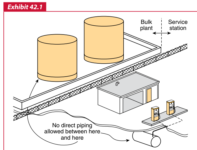
Diagram illustrating the separation requirements of the dispensing facility from the bulk plant.
