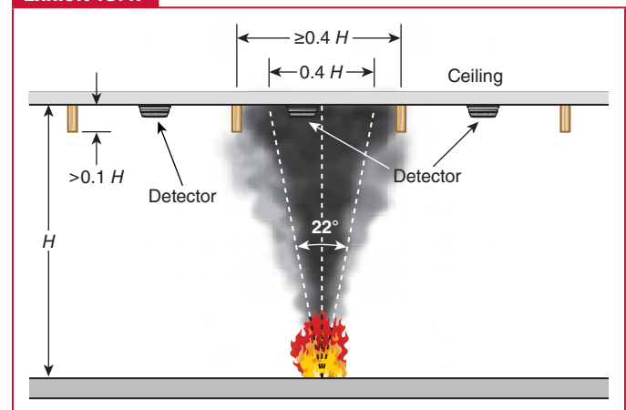
Smoke detector spacing with beam depths greater than 0.1 H and spaced more than 0.4 H .
