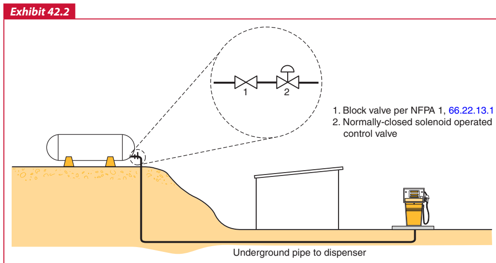
Fuel storage tank that can impose a gravity head on the dispensers.
