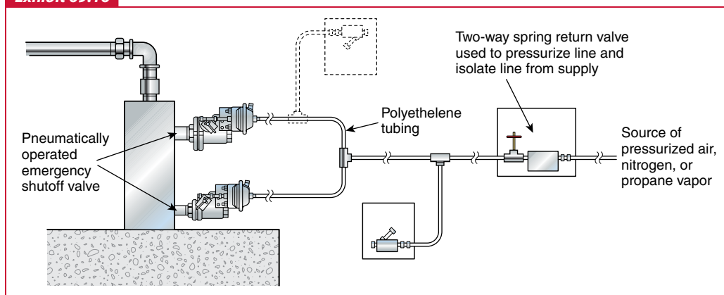
Installation of pneumatically operated emergency shutoff valve. (Courtesy of National Propane Gas Association)
