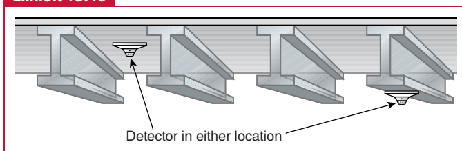
Smoke detector spacing with beams less than 0.1 H .
