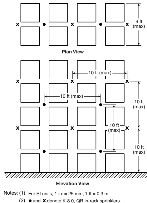
FIGURE 66.16.6.5(b) Double-Row Rack Sprinkler Layout I — Option #1. [30: Figure 16.6.5(b)]
