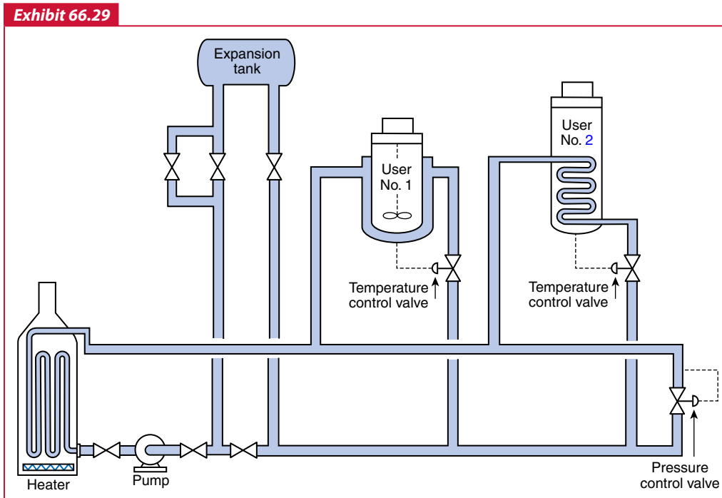
Schematic of a recirculating heat transfer system.
