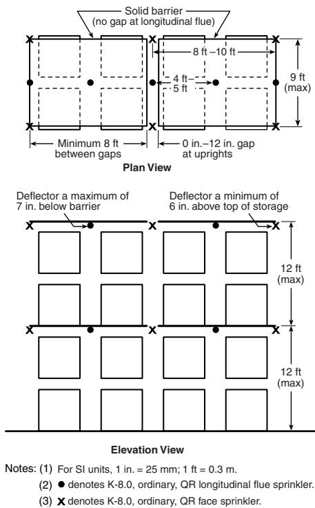
FIGURE 66.16.6.1(b) Double-Row Rack Sprinkler Layout for Design Scheme “A.” [30: Figure 16.6.1.1(b)]
