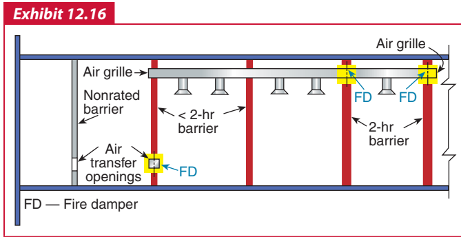
Fire damper requirements of NFPA 90A for HVAC penetrations of fire barriers.
