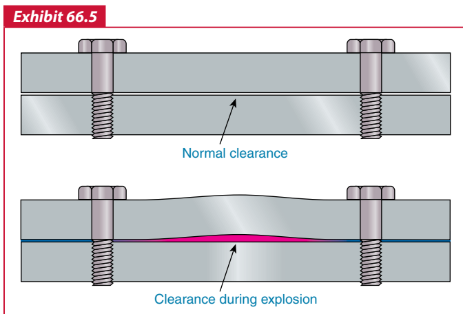
Effect of internal explosion (bottom) on cover-to-body joint clearance in an explosionproof enclosure. (Courtesy of UL LLC)
