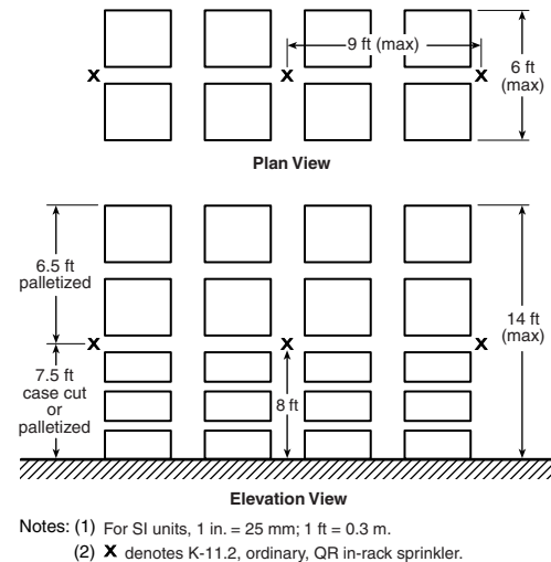
FIGURE 66.16.6.5(a) Double-Row Rack Sprinkler Layout G. [30: Figure 16.6.5(a)]
