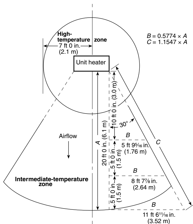
Δ FIGURE 13.3.1.9 High-Temperature and Intermediate-Temperature Zones at Unit Heaters. [13:Figure 8.3.2.5]
