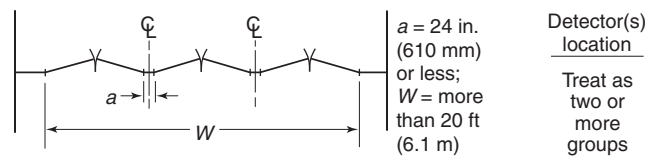
FIGURE 17.7.5.6.5.3(C) Detector(s) Location ±24 in. (610 mm) Requirements for Group Doorways over 20 ft (6.1 m) in Width.
