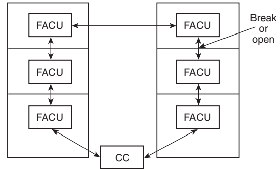
FIGURE F.3.14(i) Style 7 Fiber Network (Two LANs).
