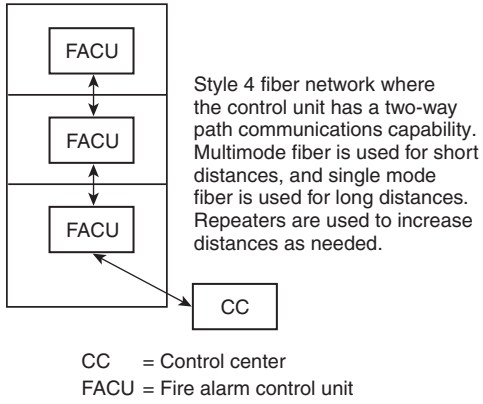
FIGURE F.3.14(f) Style 4 Fiber Network.
