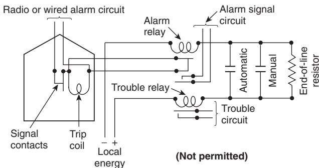
FIGURE A.27.6.3.2.1(2)(b) Shunt-Type Auxiliary Alarm System (Not Permitted).
