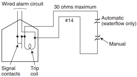
FIGURE A.27.6.3.2.1(2)(a) Shunt-Type Auxiliary Alarm System (Permitted).
