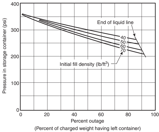
▲ FIGURE H.1(c) Calculated Pressure Recession for 360 psi Storage.
