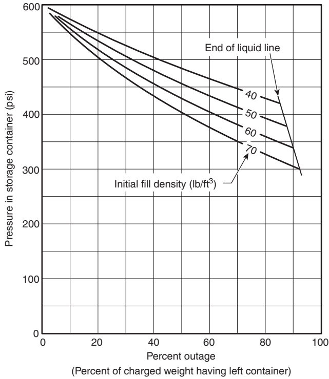
▲ FIGURE H.1(b) Calculated Pressure Recession for 600 psi Storage.
