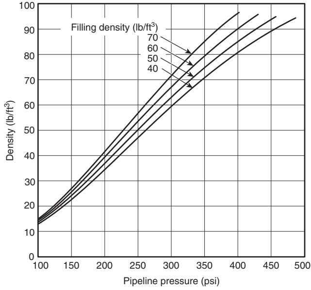
N FIGURE H.1(f) Pipeline Density for 600 psi Systems Based on Constant Enthalpy Expansion.
