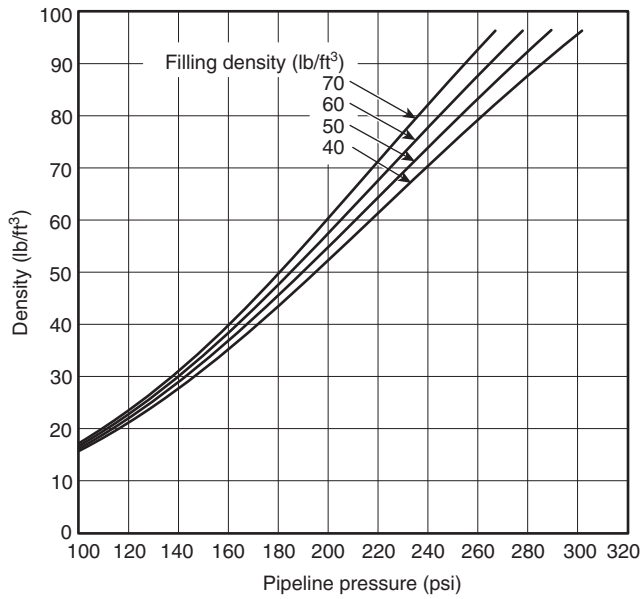
N FIGURE H.1(g) Pipeline Density for 360 psi Systems Based on Constant Enthalpy Expansion.
