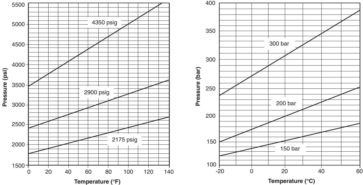
▲ FIGURE A.4.1.4.1(1) Isometric Diagram of IG-55 Filled at 59°F (15°C).
