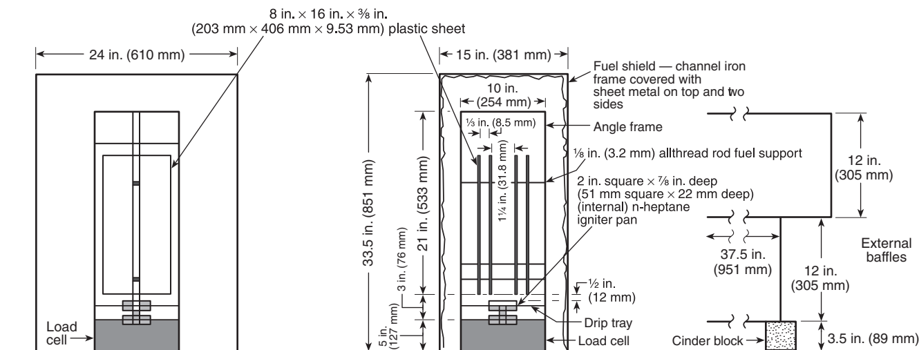
FIGURE A.5.4.2(a) Four-Piece Modified Plastic Setup.
