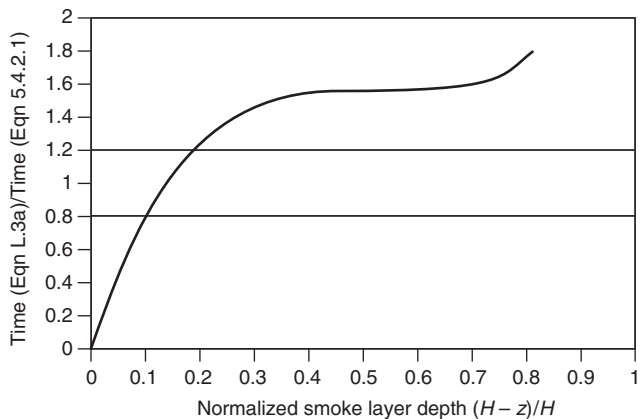
FIGURE L.3(b) Comparison of Algebraic Equations, Equations 5.4.2.1 and L.3a: Steady Fire — Normalized Smoke Layer Depth.
