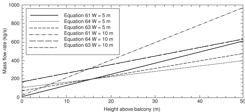
FIGURE A.5.5.2.10 Estimated Mass Flow Rates.
