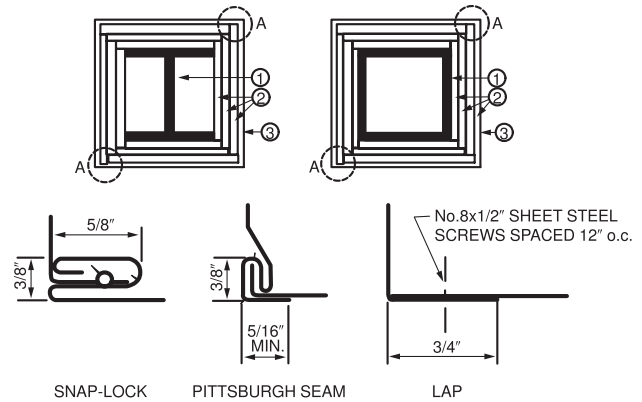
FIGURE 722.5.1(2) GYPHUM-PROTECTED STRUCTURAL STEEL COLUMNS WITH SHEET STEEL COLUMN COVERS
