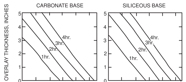
FIGURE 722.2.2.2 FIRE-RESISTANCE RATINGS FOR TWO-COURSE CONCRETE FLOORS
