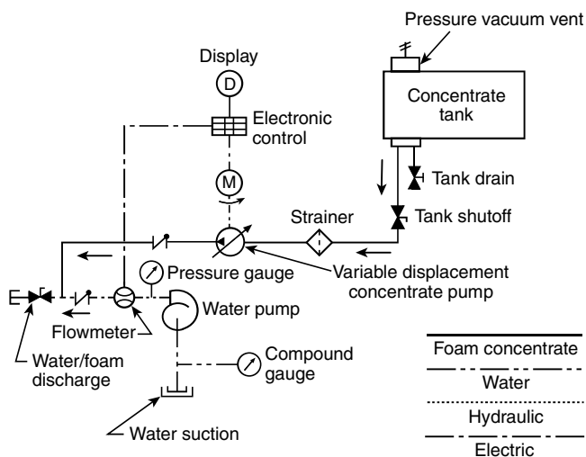
FIGURE A.3.3.24.3(a) Single-Meter Flow-Sensing Direct Injection Foam Proportioning System.
