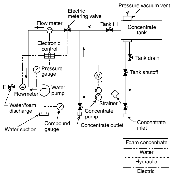
FIGURE A.3.3.24.3(b) Dual-Meter Flow-Sensing Direct Injection Foam Proportioning System.
